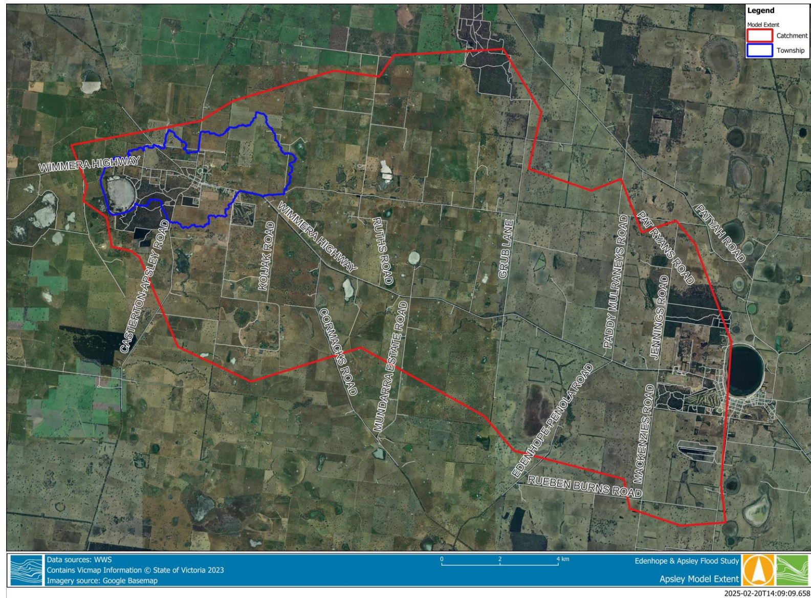
Figure 2-1 Model Schematic - Apsley
