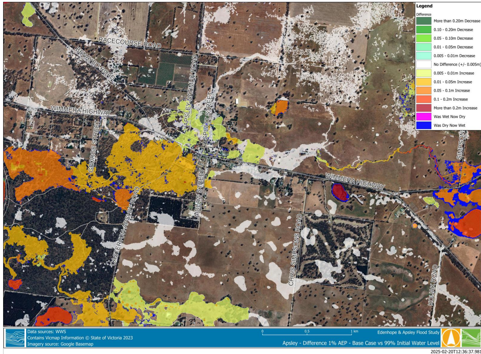
Figure 3-5 Difference Plot for 1% AEP - Base Case vs 99% Initial Water Level
