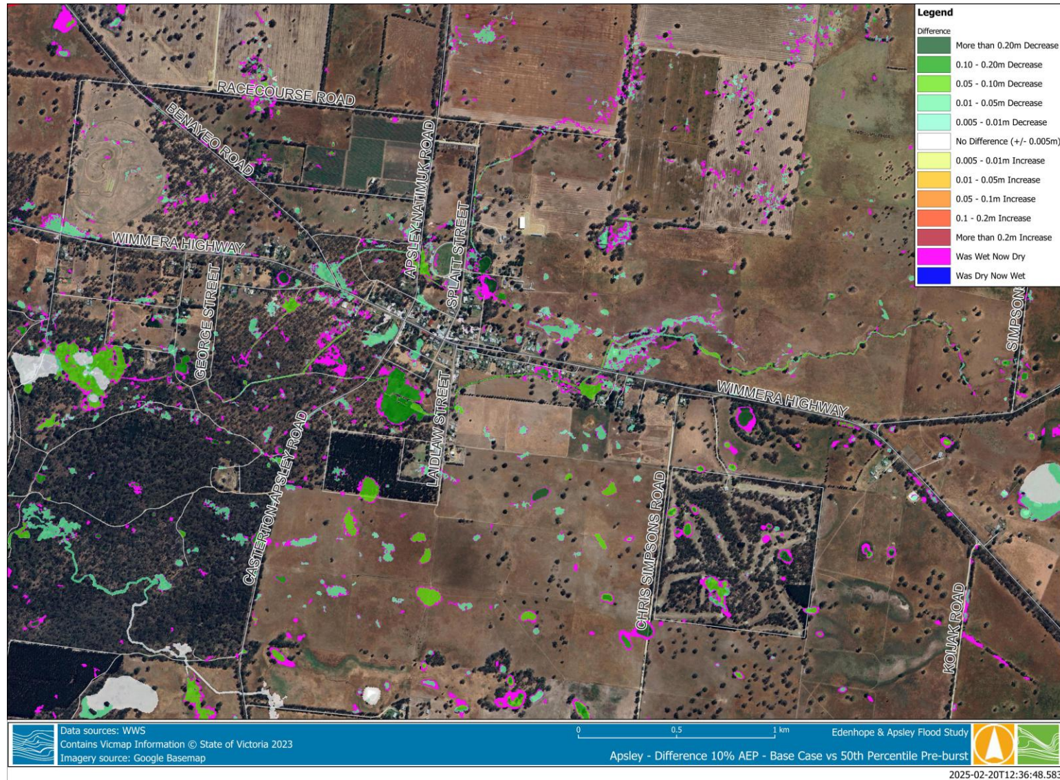
Figure 3-10 Difference Plot for 10% AEP – Base Case vs 50th Percentile Pre-burst
