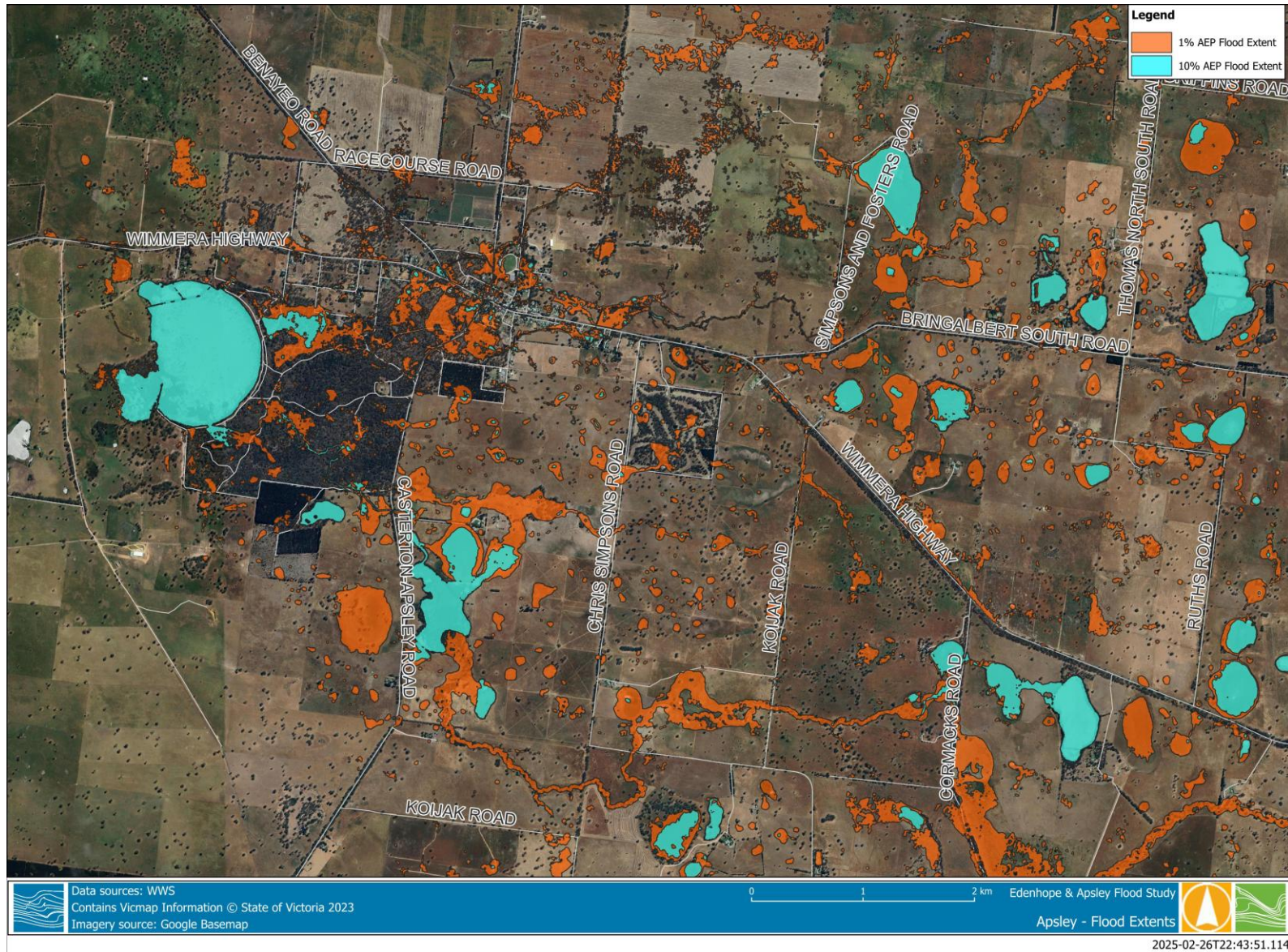
Figure 4-3 Broad extent – 10% and 1% AEP flood events
