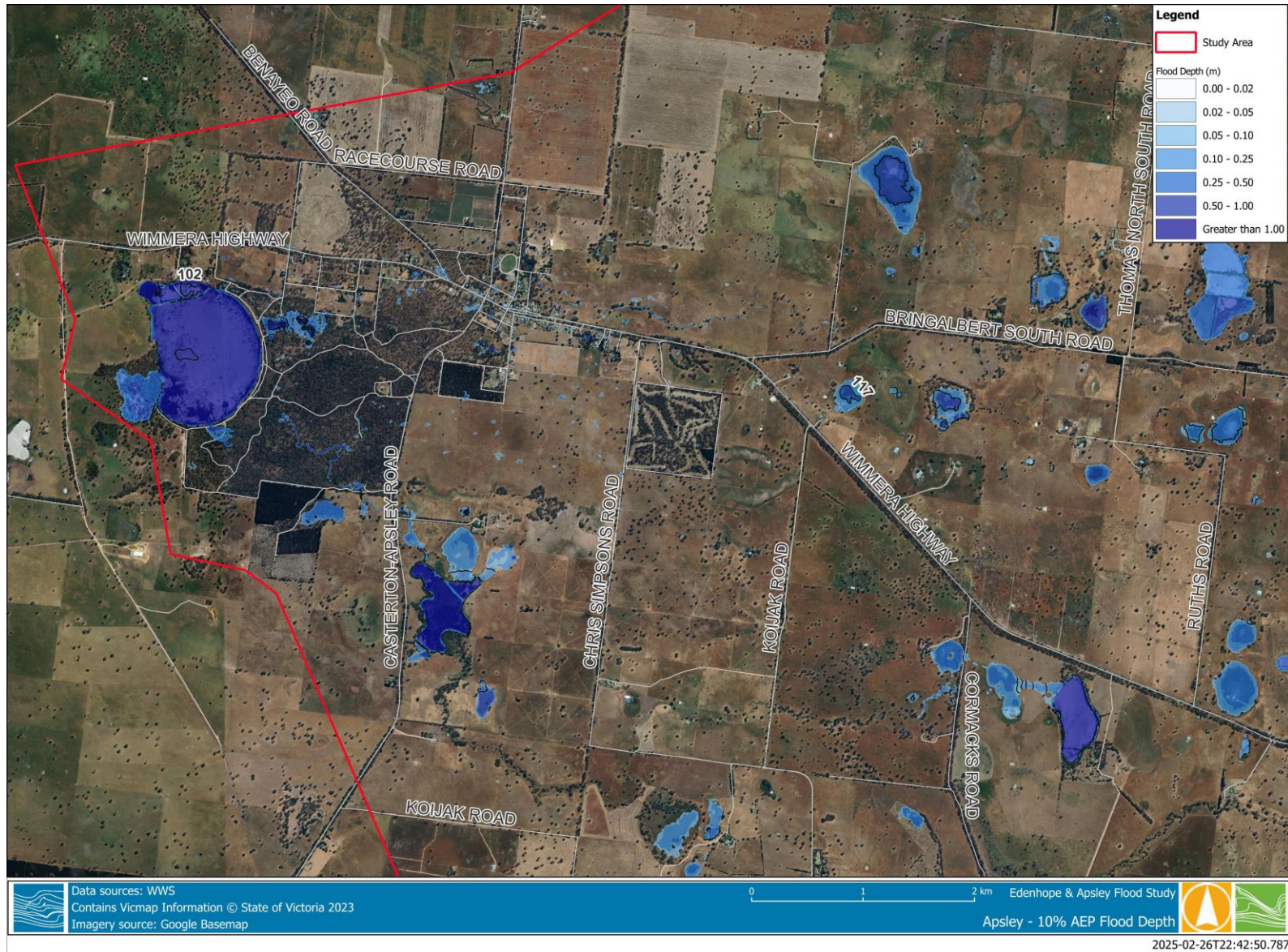
Figure 4-9 Broad extent - 10% flood depth with water surface elevation contours
